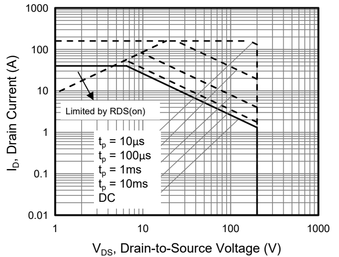
Figure 4. Safe Operation Area For TO-220/3P/247
