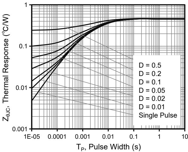
Figure 3. Transient Thermal Impedance For TO-220/3P/247
