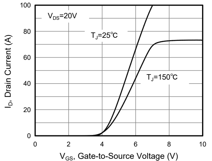
Figure 6. Transfer Characteristics
