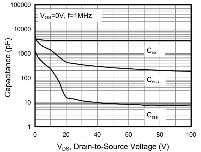
Figure 8. Capacitance
