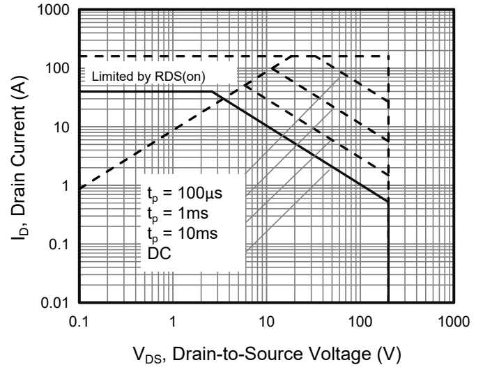
Figure 2. Safe Operation Area For TO-220F, TO-220FT
