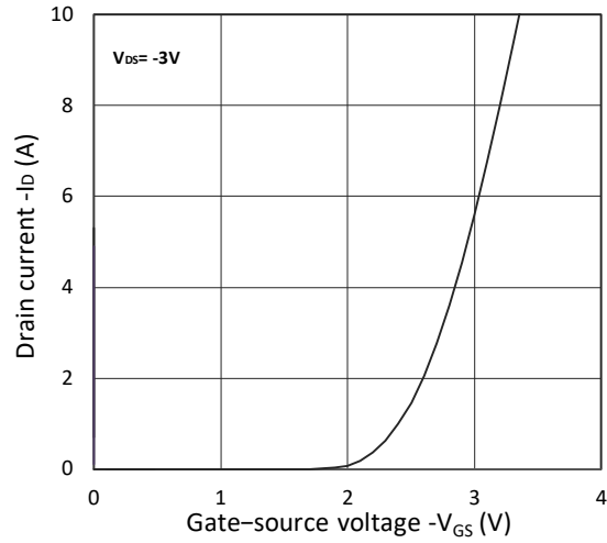
Figure 2. Transfer Characteristics
