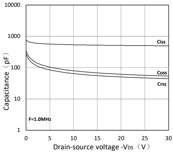
Figure 7. Capacitance Characteristics
