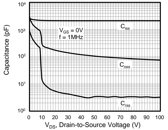
Figure 8. Capacitance
