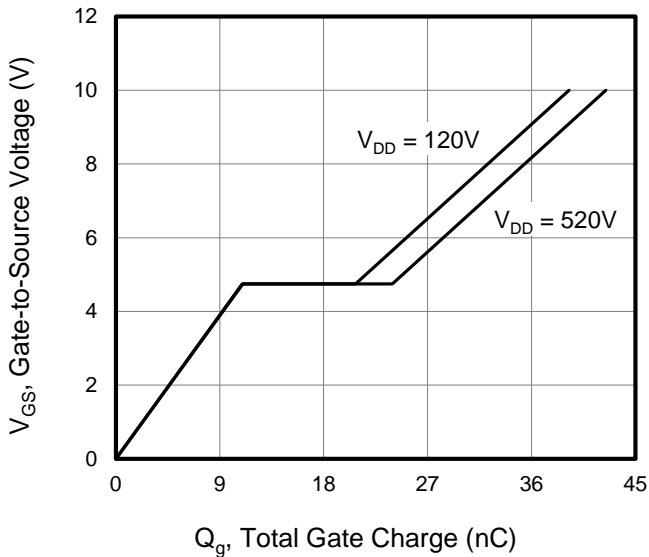
Figure 9. Gate Charge
