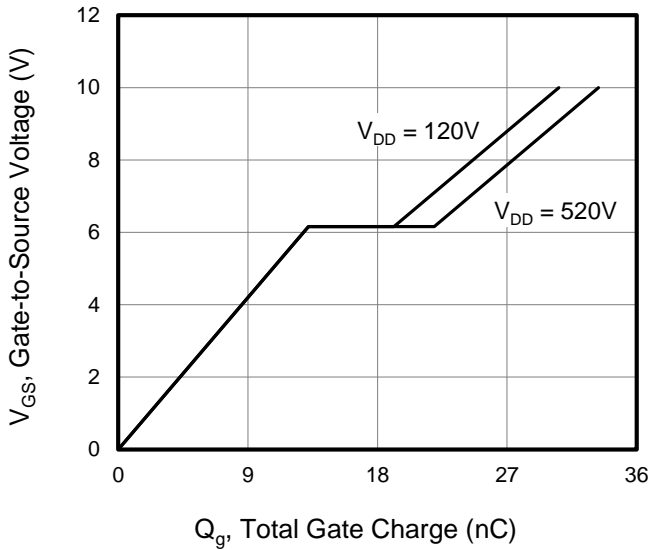
Figure 9. Gate Charge
