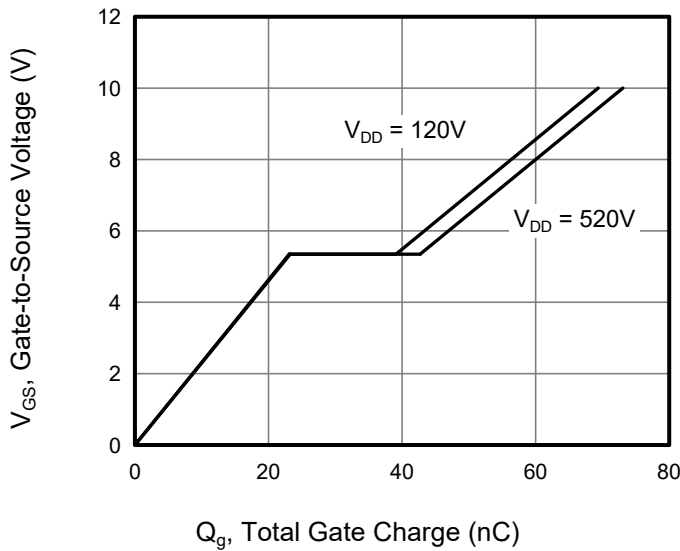
Figure 9. Gate Charge
