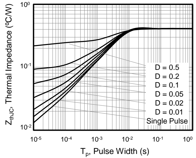
Figure 2. Transient Thermal Impedance For TO-3P/247
