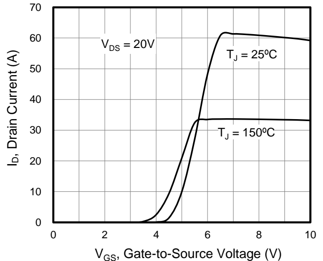
Figure 6. Transfer Characteristics
