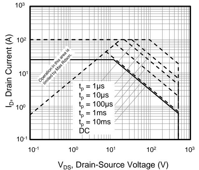
Figure 4. Safe Operation Area For TO-3P/247
