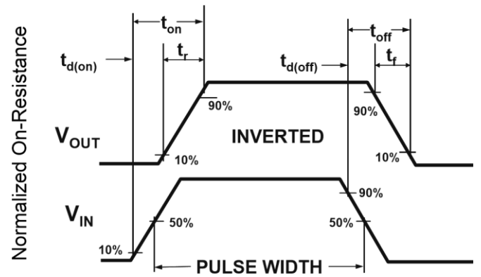
Figure 2: Switching Waveforms
