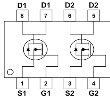
SOP8 Pin Configuration
