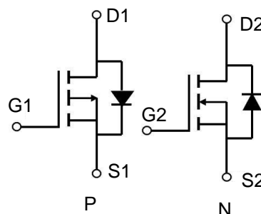
SOT 23-6L Pin Configurations
